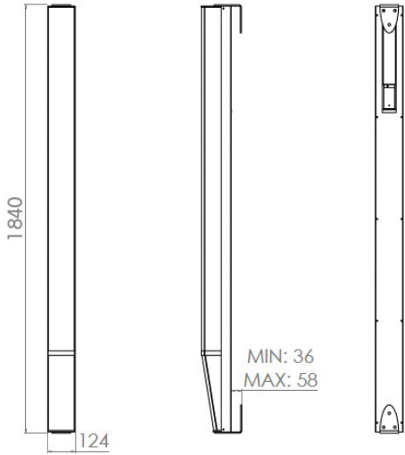
Front views
